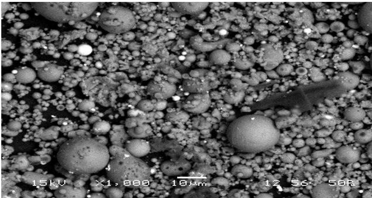
SEM Analysis of Fly ash at 1000 magnification
